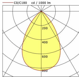
Flixx 300 Square (FLIQZ 300.25, 1xLED 21W 830/3000K 2040lm)
